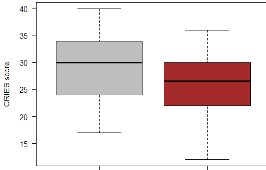
Boxplot of Pre-and Post CRIES scores
